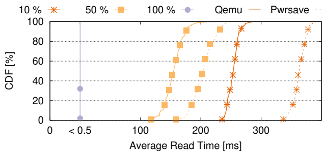
Fig. 6. Read time (CDF) from secure storage using MQTT-TZ’s secure cache for different numbers of cached objects. The cache capacity grows from 10% up to 100% of the total objects. Dashed lines represent hardware results and bold lines emulated ones.
